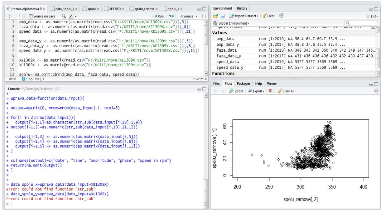
Fig. 2. R-studio software
