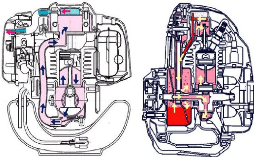
Fig. 3. Visualization of Honda GX 25 motor
