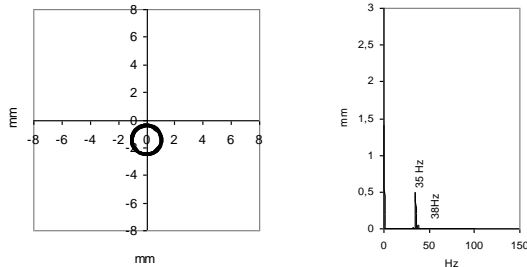
Fig. 7. Trajectory of movement and amplitude-frequency characteristic of the speed of vibration of the mass center of the rotor after balancing
